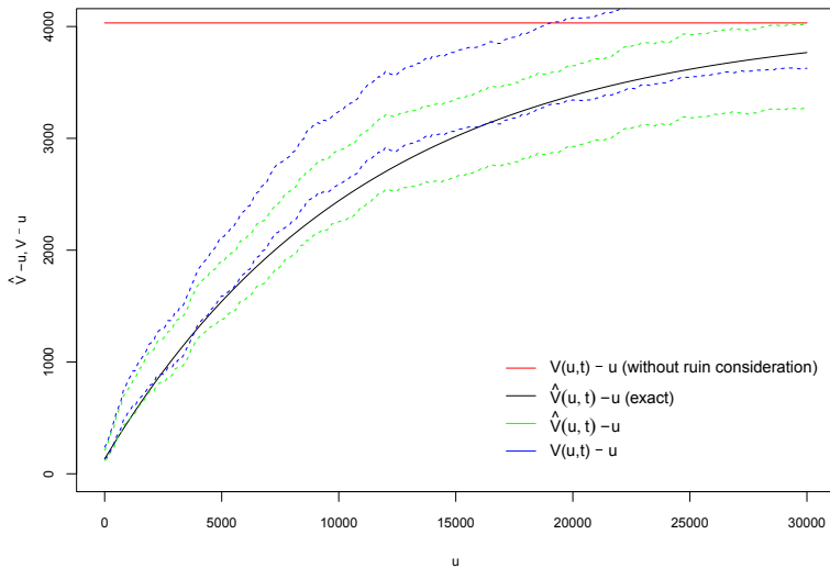
Figure 7: \hat{V}(u, t) - u as a function of u and simulated \hat{V}(u, t) - u and V(u, t) - u with their 95% confidence interval bound in dashed. Both jumps are exponentially distributed.
